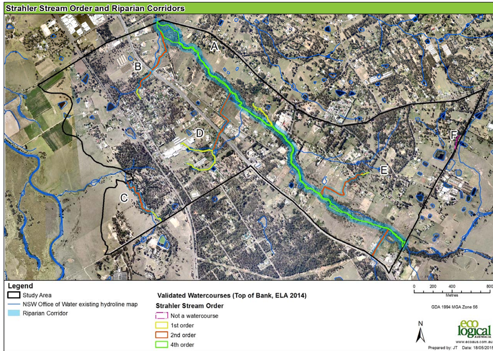
Figure 10: Strahler stream order and corresponding riparian corridors
