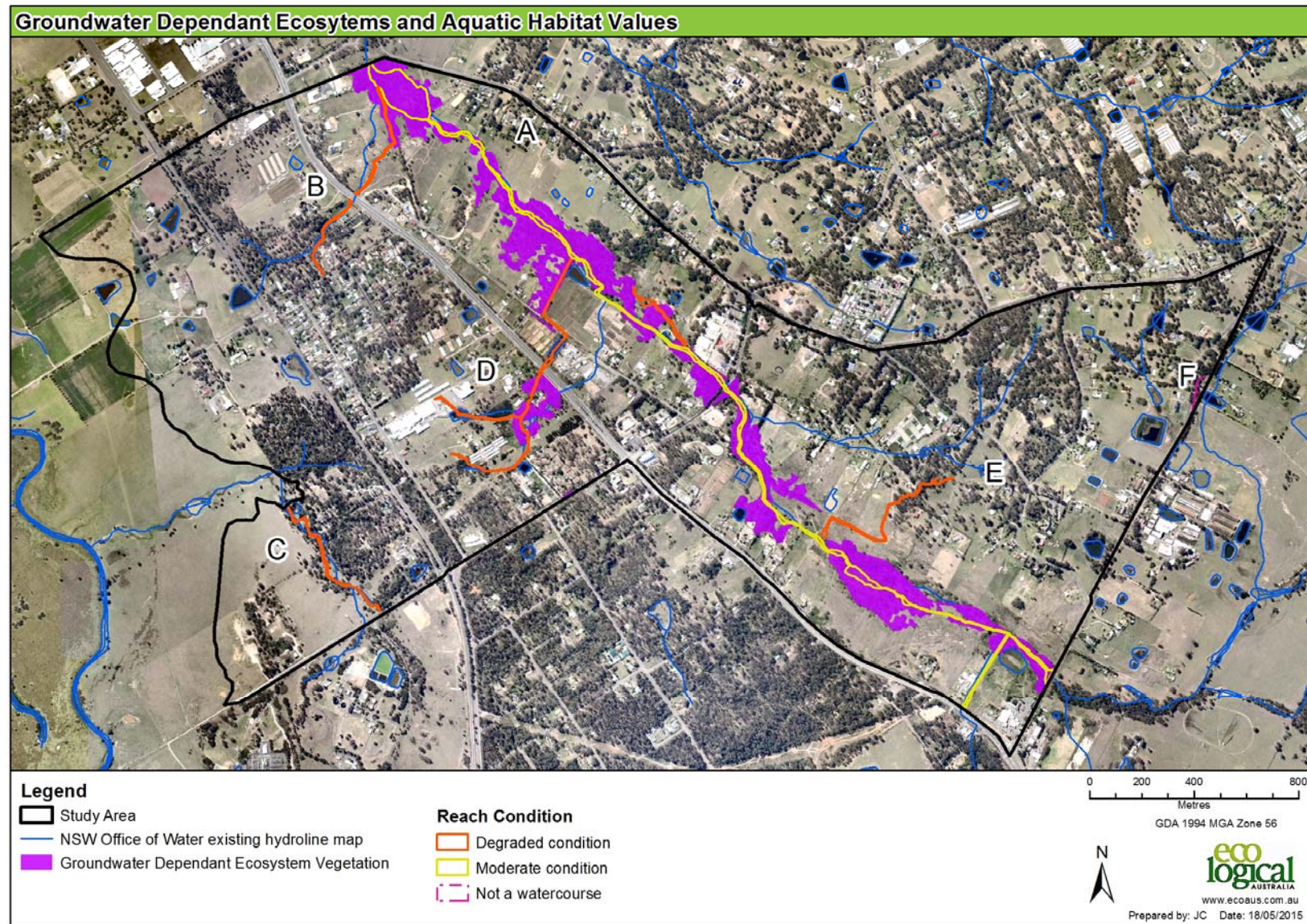
Figure 11: Groundwater Dependant Ecosystem and Aquatic Habitat values
